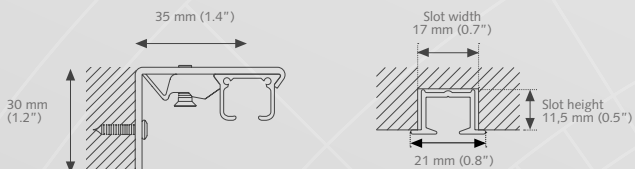
Milling dimensions KS Recess
